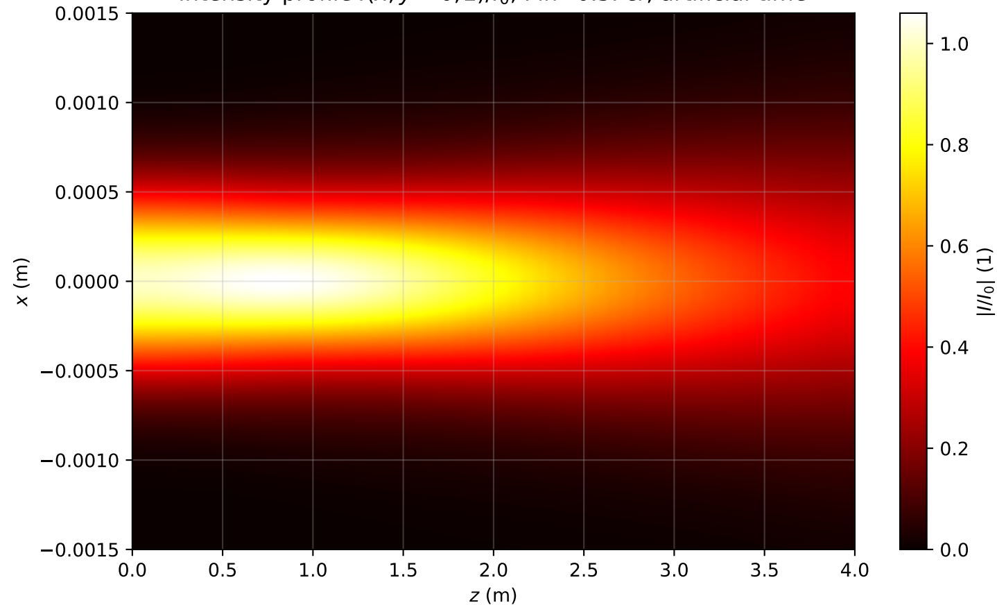
Intensity profile I(x, y = 0, z)/I_0 , P_{in}=0.5P_{cr} , artificial time
